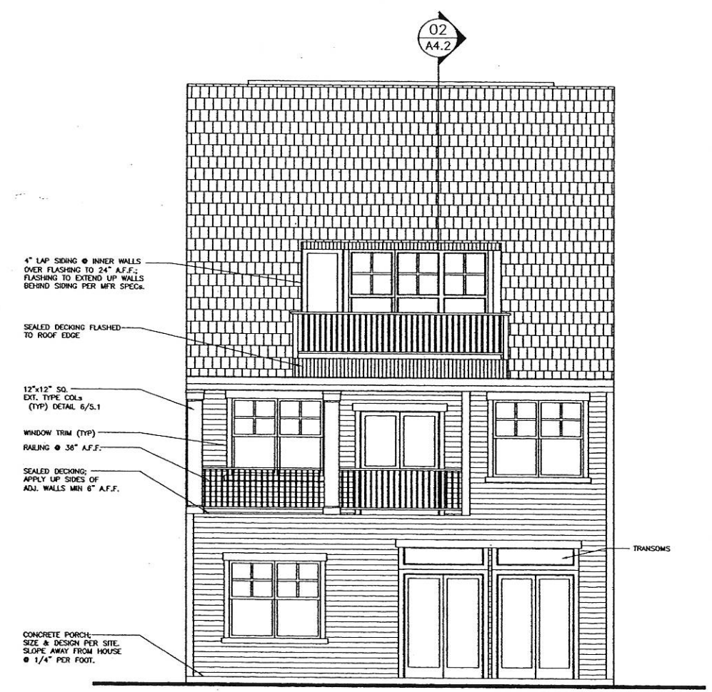
02 REAR ELEVATION 1/4" = 1'-0" (1/8" = 1'-0" @ 11x17)
