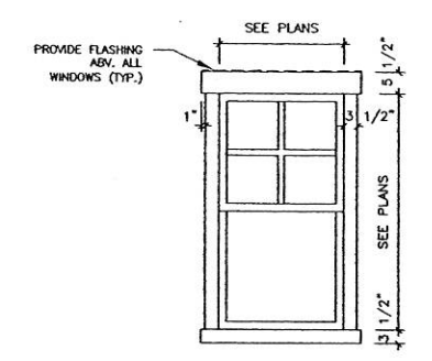
03 TYP. WINDOW TRIM DETAIL SCALE: 1/2" = 1'-0" (1/4" = 1'-0" @ 11x17)
