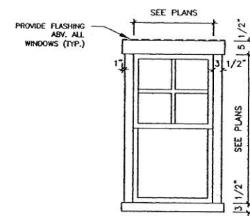
03 TYP. WINDOW TRIM DETAIL SCALE 1/2" = 1'-0" (1/4" = 1'-0" F 11x17)
