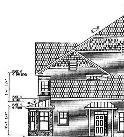
05 OPT. SIDE ELEVATION 1/8" = 1'-0" (1/16" = 1'-0" F 11x17)
