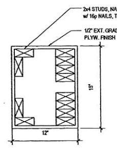
08 DETAIL - Column 1 1/2" = 1'-0"
