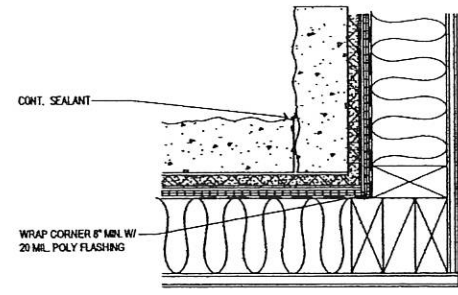
03 DETAIL - Stone @ Inside Corner 3" = 1'-0"
