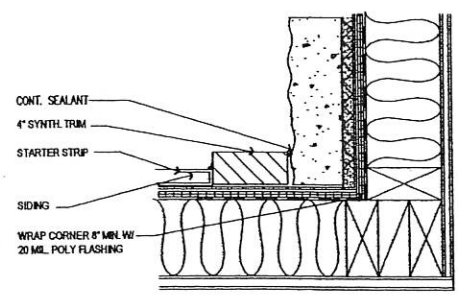
04 DETAIL - Stone/Siding @ Corner
