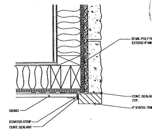
02 DETAIL - Stone/Siding @ Corner 3" = 1'-0"
