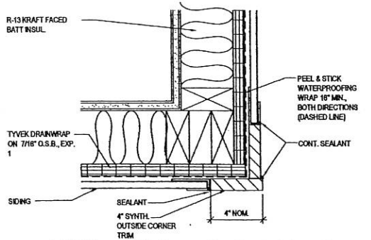
05 DETAIL - Siding @ Outside Corner 3" = 1'-0"
