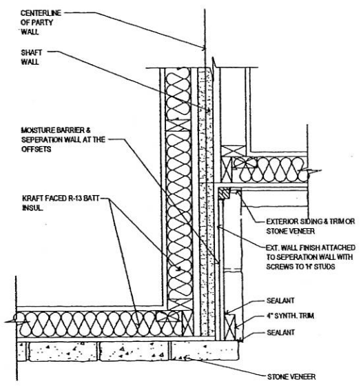
01 DETAIL - Party Wall @ Offset
