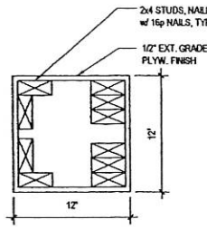
09 DETAIL - Column 1 1/2" = 1'-0"
