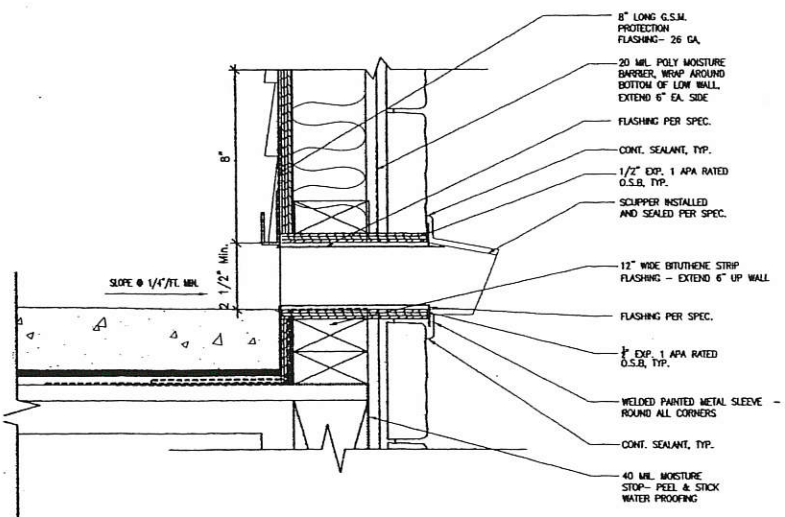
03 DETAIL - Scupper @ Balcony - Unit A
