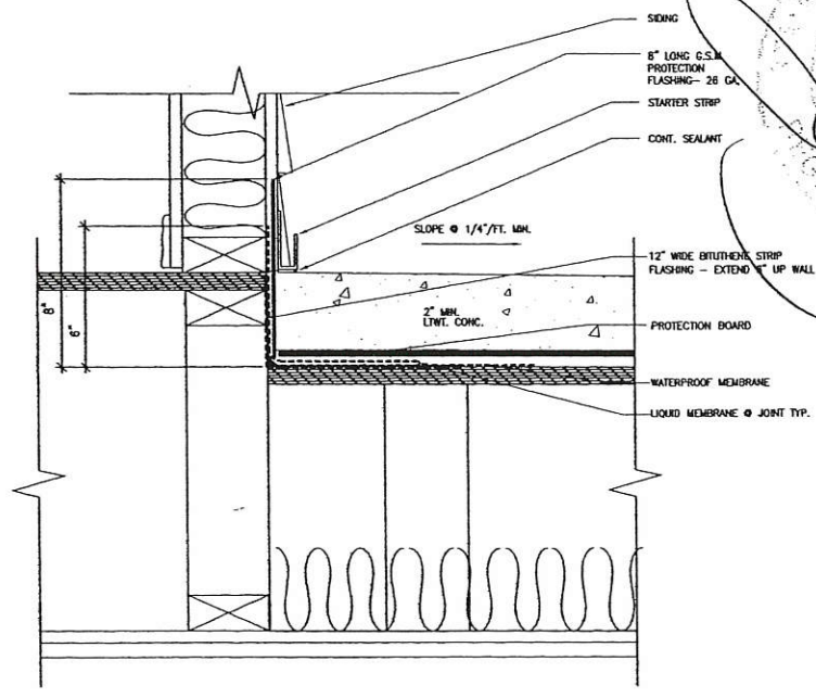
01 DETAIL - Balcony @ Unit A
