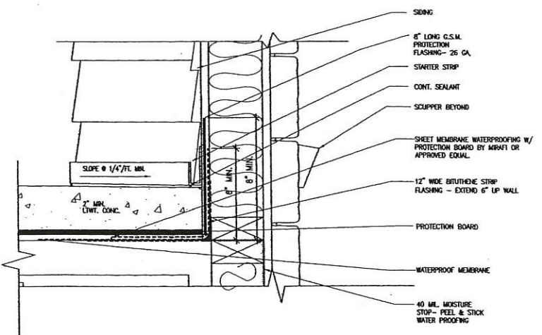
02 DETAIL - Balcony Edge @ Unit A
