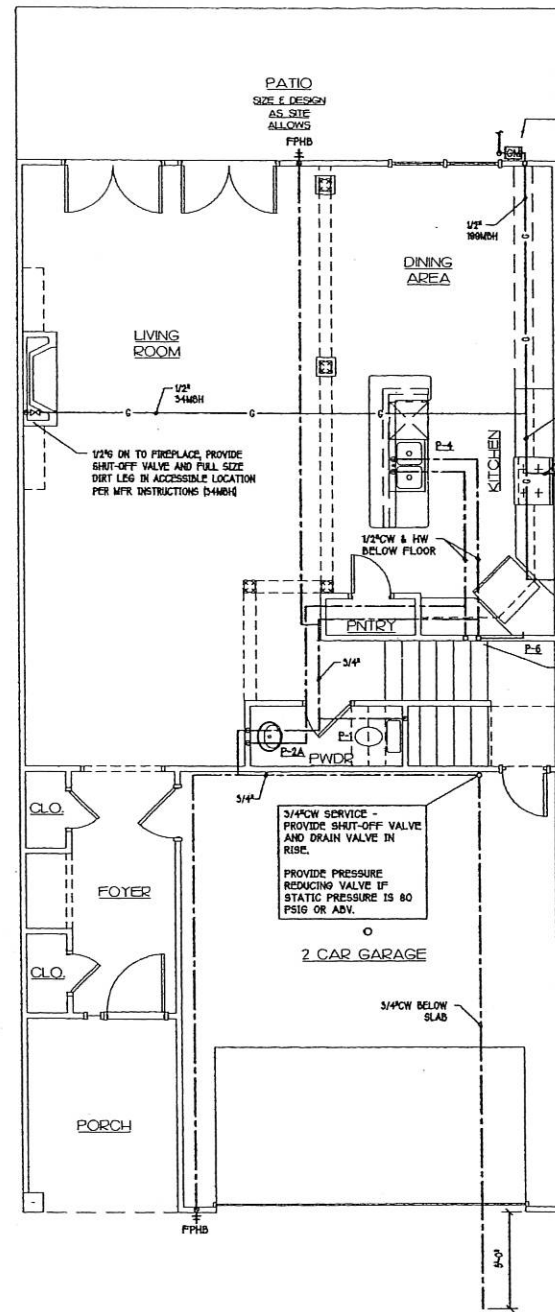
1 FIRST FLOOR THREE STORY UNIT WATER & GAS PLAN P4 1/4" = 1'-0"
